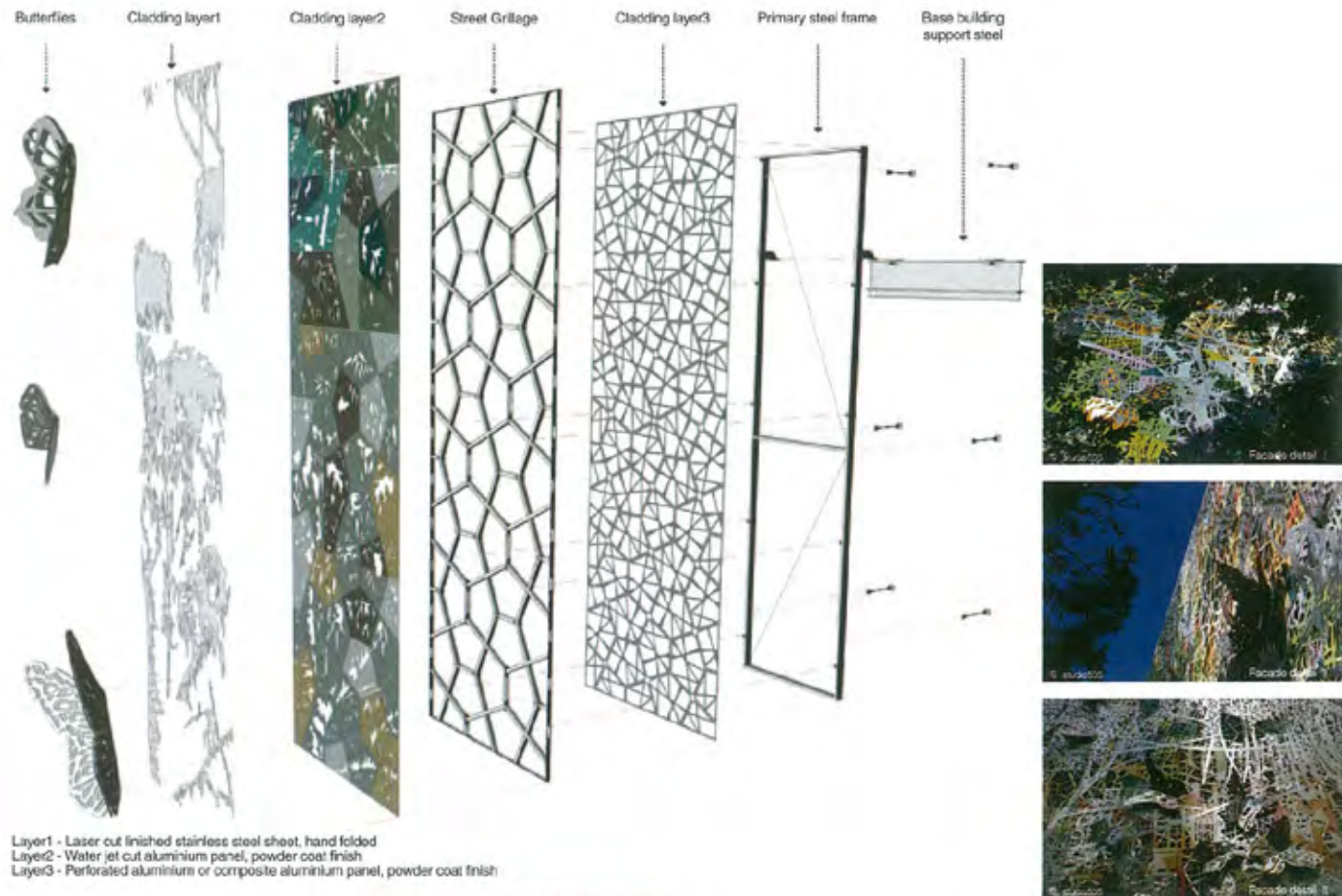
Exploded perspective of facade cladding
